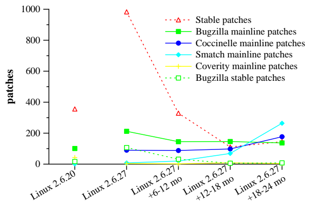
Figure 1. Various kinds of patches applied to the stable kernels 2.6.20 and 2.6.27 and to the mainline kernel in the same time period
