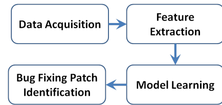
Figure 2. Overall Framework
