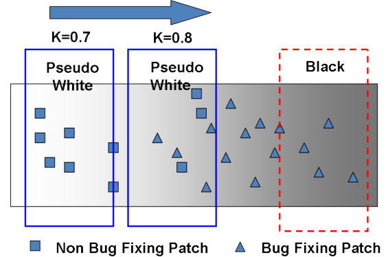
Figure 5. Effect of Varying k . The pseudo white data is the bottom k commits that we treat as a proxy to non bug fixing patches. The three boxes corresponding to pseudo white (2 of them) and black represent the aggregate features of the respective pseudo-white and black data in our training set respectively. The squares and triangles represent test data points whose labels (i.e., bug fixing patches or not) are to be predicted.
