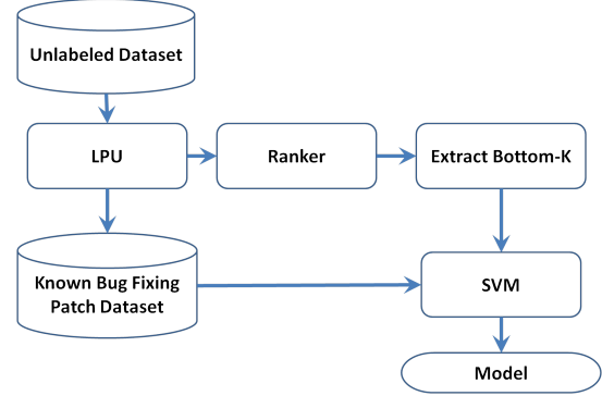
Figure 4. Model Learning
