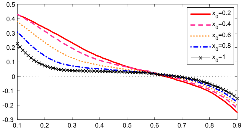
Figure 7. Bias functions implied by the in-fill asymptotic distribution given in Theorem 4.1 when \beta_1 = 1 and \beta_2 = 1.03 with various initial conditions.
