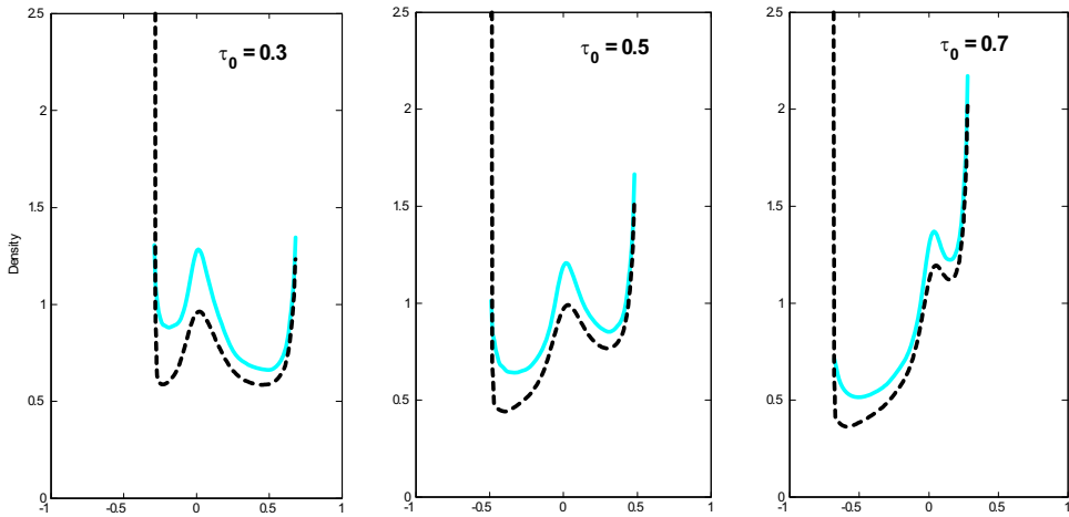
Figure 2. Densities of \hat{\tau}_{ML} - \tau_0 given in Eq. (7) when \kappa = 138, \delta = -20, \sigma = 1 and \tau_0 = 0.3, 0.5, 0.7 , respectively. Solid lines are densities for x(0) = 0.2 ; broken lines are densities for x(0) = 1 .
