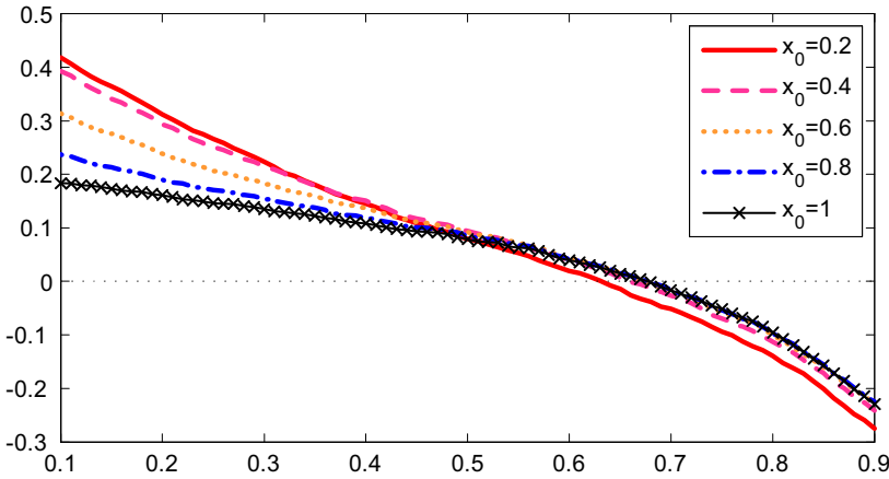
Figure 6. Bias functions implied by the in-fill asymptotic distribution given in Theorem 4.1 when \beta_1 = 0.9 and \beta_2 = 1 with various initial conditions.
