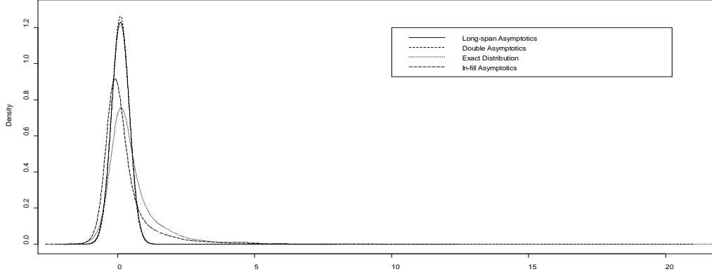
Figure 2: Four densities of \hat{\kappa} when \kappa = 0.1 , h = 1/12 and T = 2 .
