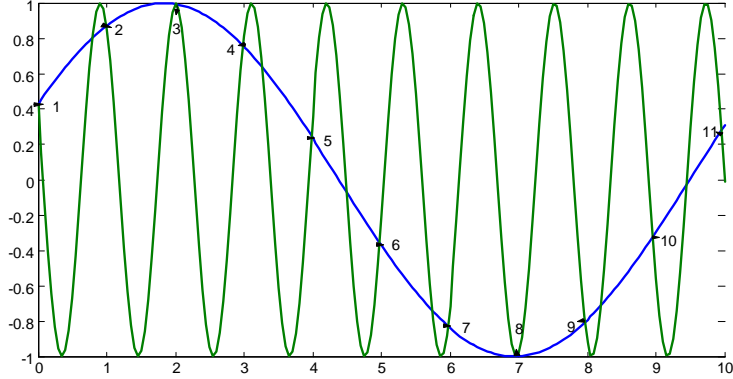
Figure 1: Aliasing problem. Arrows represent a set of discrete samples whose sampling interval is 1.
