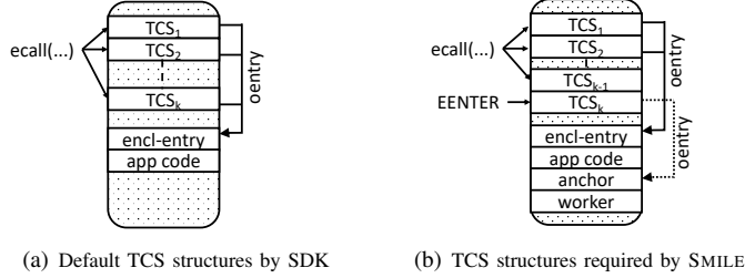
Fig. 7. Comparison between the default TCS setup and the one for SMILE where TCS_k is different from others.
