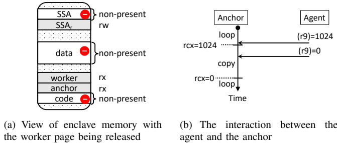
Fig. 5. Worker Integrity Checking
