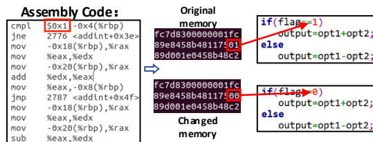
Fig. 9. Memory analysis of enclave code with SMILE.
