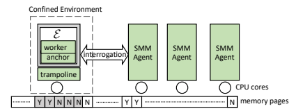
Fig. 1. A system view of confined interrogation. Grey boxes represent EPC pages of \mathcal{E} . Only Pages labelled with ‘Y’ are accessible to \mathcal{E} .
