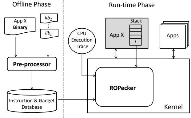
Figure 1. The architecture of ROPEcker. The shaded square represents a protected application.
