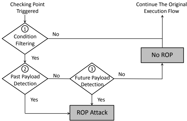
Figure 3. The ROP checking logic.
