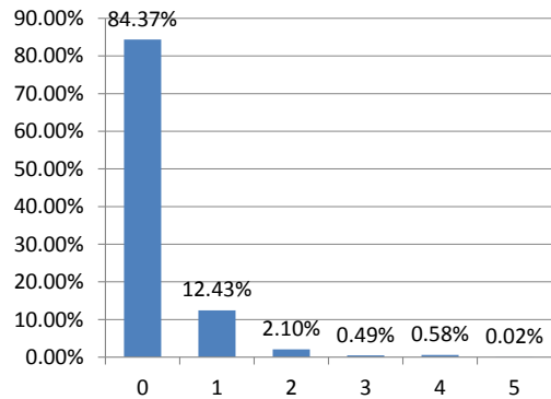
Figure 4. The length of payload measurement results. The number (0 to 5) is the payload length. In the major cases (84.37%), there is no gadget identified at all.
