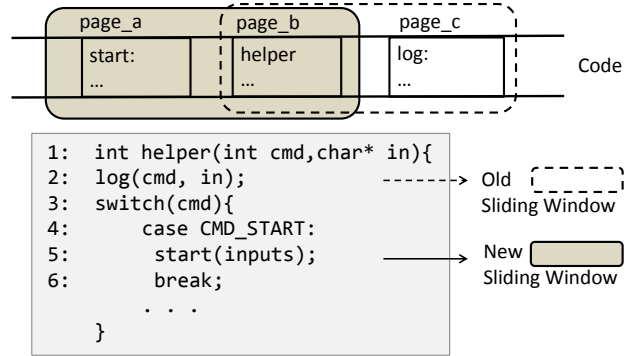
Figure 2. The sliding window and its update. In this example, the size of the sliding window is 2 pages. When the execution flow reaches to log function (line 2), the sliding window is ( page_b , page_c ). Later the window is updated to ( page_a , page_b ) when the start function (line 5) is executed. Note that the code pages in the sliding window can be non-contiguous.
