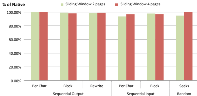
Figure 6. The disk performance results.
