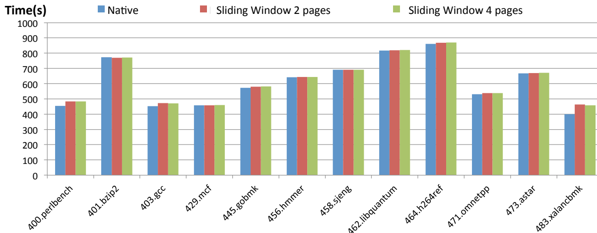
Figure 5. The SPEC INT2006 Benchmark Results.
