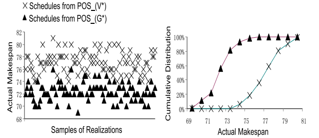
(a) Results of PSP50 from J10 under \epsilon = 0.2
