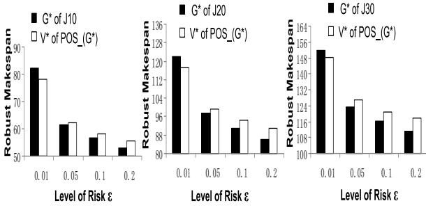
Figure 2: Comparison of G^* and V^* of POS_{G^*} under \sigma = 1.5 .
