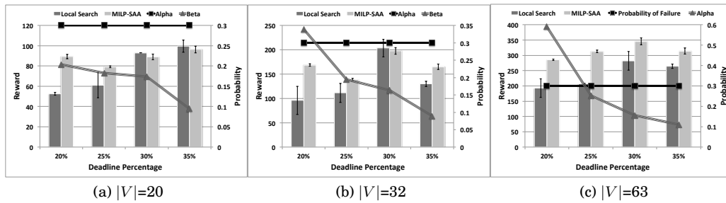
Fig. 1: Plots showing accumulated reward by our approaches as deadline percentage is varied. In all three graphs: x -axis represents the deadline percentage. Primary y -axis represents the reward accumulated and secondary y -axis represents the probability of failure. The two bars correspond to the reward (primary y -axis) accumulated by Local Search and MILP-SAA methods. The two lines correspond to the desired (Alpha) and actual (Beta) probability of failure (secondary y -axis) values. We also provide error bars representing variance on reward values across multiple runs.
