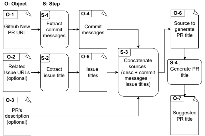
Fig. 1. The architecture of AUTOPRTITLE
