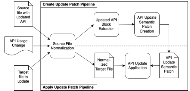
Figure 3: System overview of CocciEvolve
