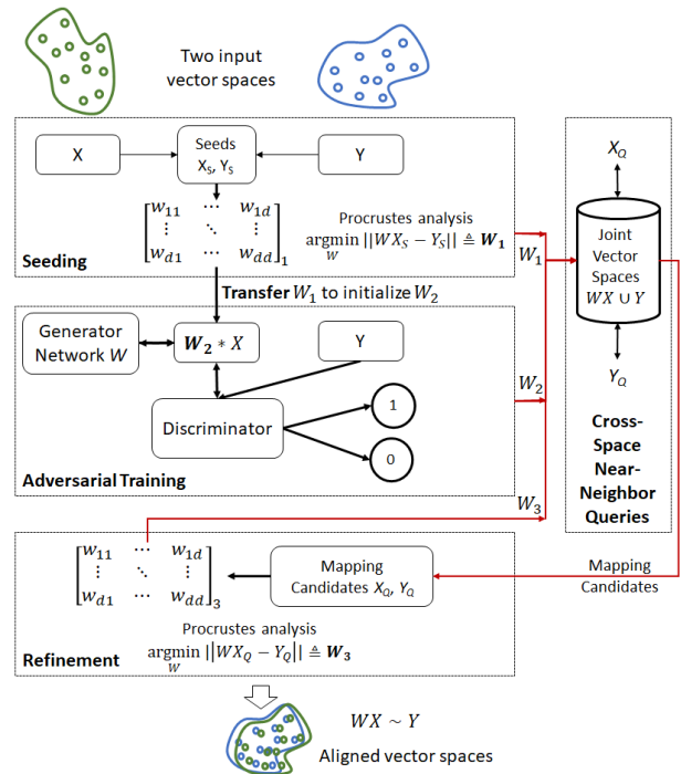
Figure 2: Domain adaptation steps to align two vector spaces
