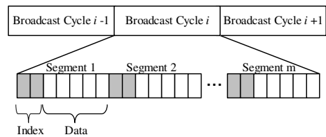
Figure 1: (1, m) scheme
