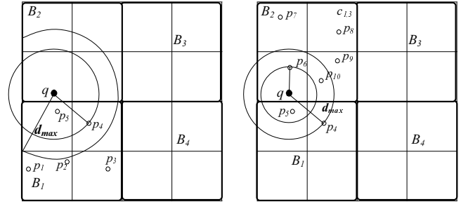
(a) Processing c_{0,0} , c_{1,0} , c_{1,1} , c_{0,1} (b) Processing c_{0,2} , c_{0,3} , c_{1,2} Fig. 8. The second step of a 2-NN computation
