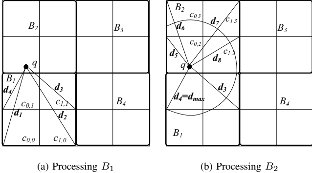
Fig. 7. The first step of a 2-NN computation
