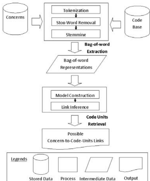
Fig. 1. Concern Localization using Information Retrieval.
