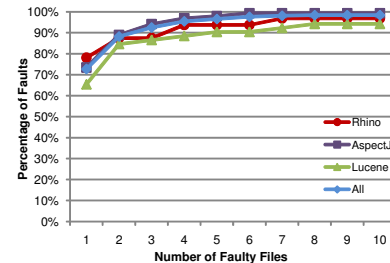
Figure 3. Proportion of faults versus file locality.
