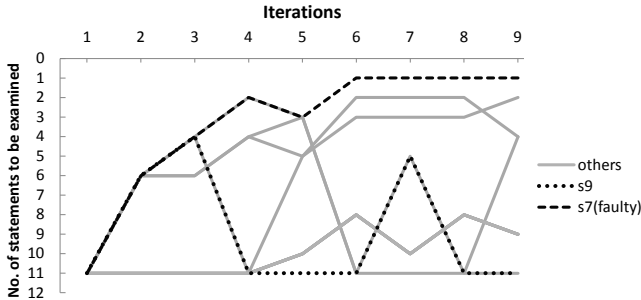
Figure 2: Motivating Example
