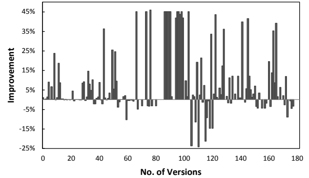
Figure 5: Improvement of DMS over FEP-ADDTL.
