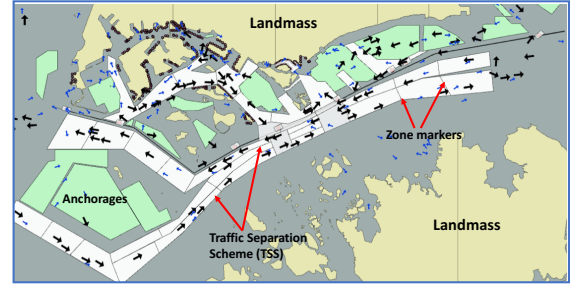
Figure 1: Electronic navigation chart (ENC) of straits near a large asian city with color-coded features (best viewed electronically)
